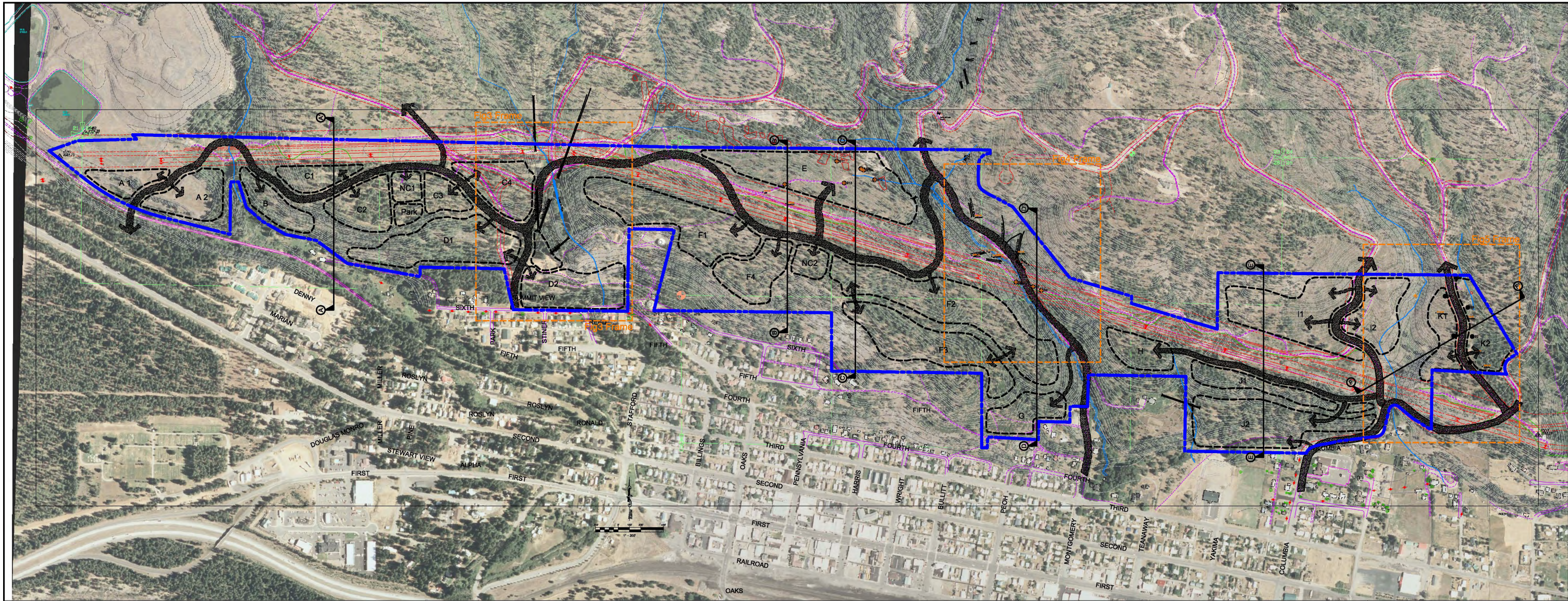
Figure 10 Sapphire Skies LLC - City Heights Site Layout Aerial with Current Contours with Building Areas
