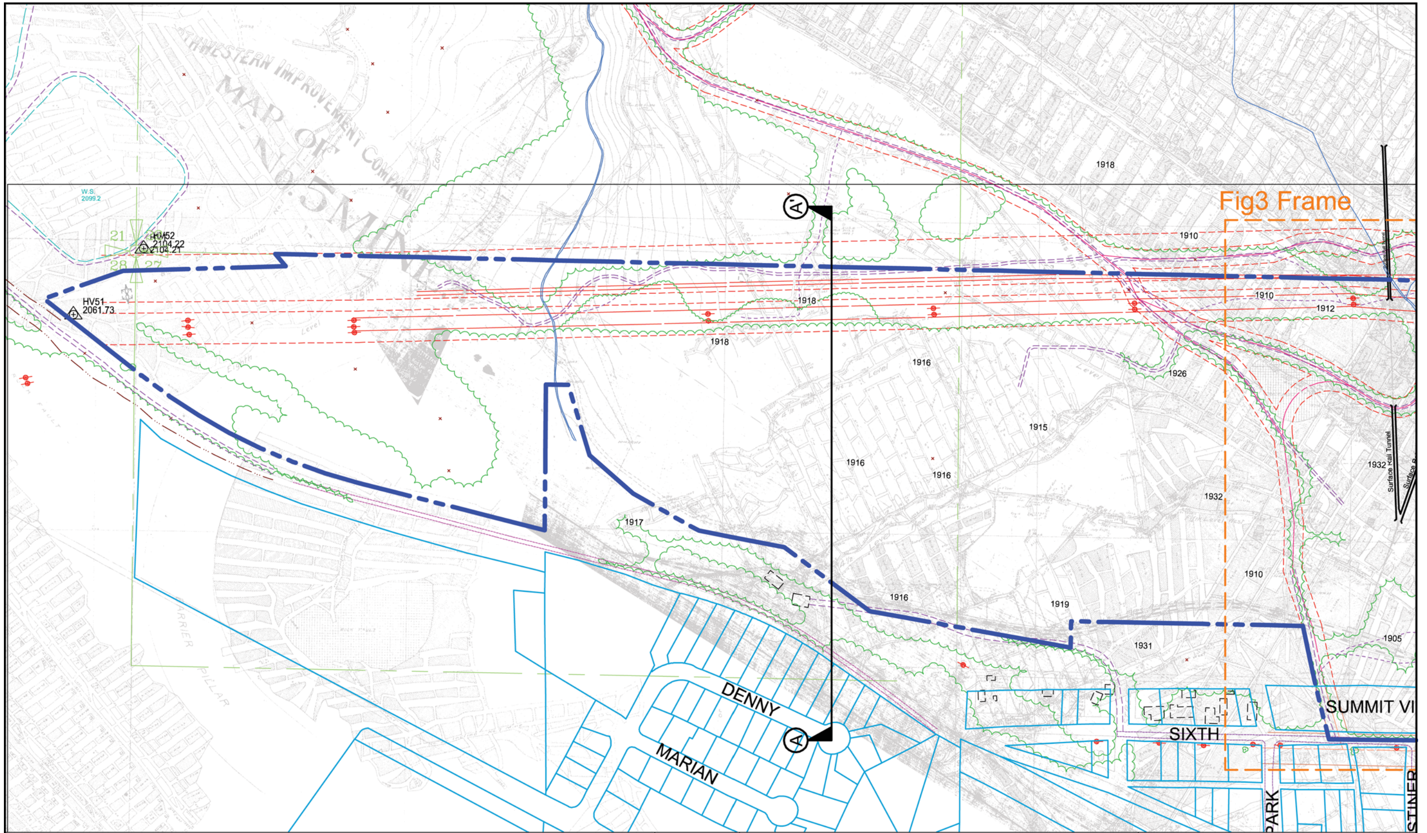
Figure 2 Sapphire Skies LLC - City Heights Site Layout with Historic Mine Workings Sheet 1 of 4
