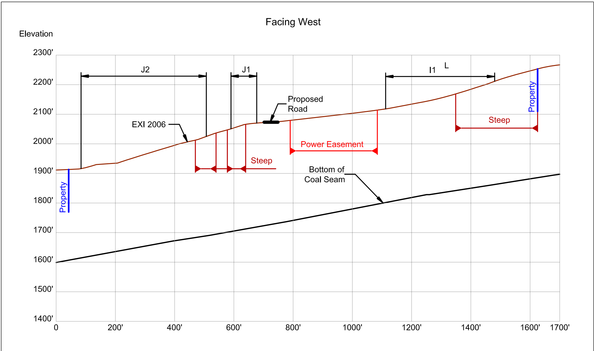
Figure 8 Sapphire Skies LLC City Heights Section E-E' Sheet 5 of 6
