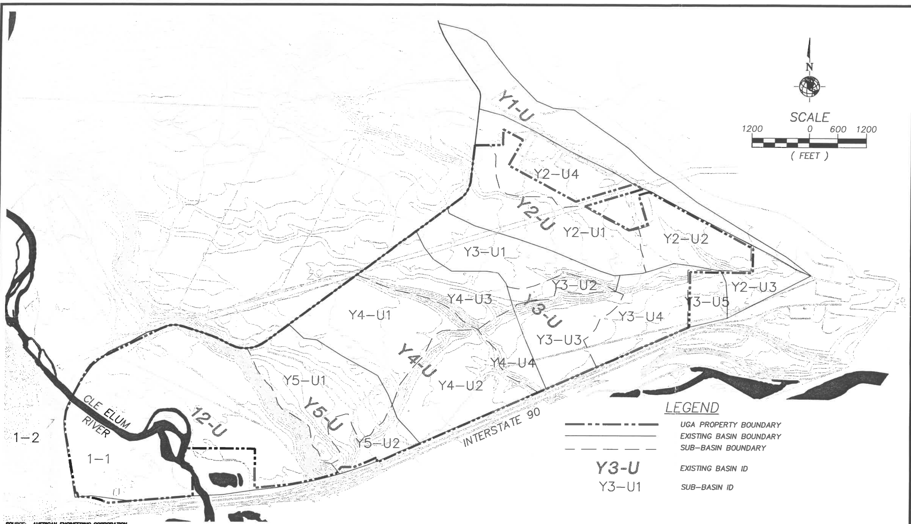
Figure 2-5 Developed Condition Basin Boundaries
