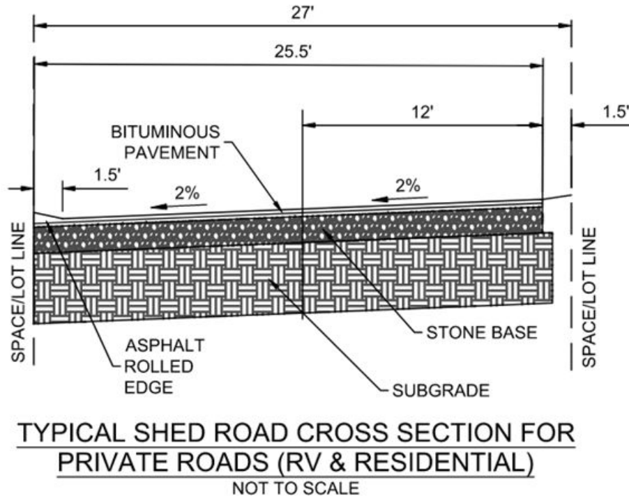
Figure 4 - Typical Private Shed Road Cross Section
