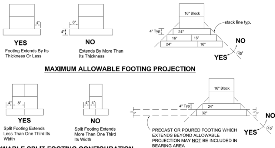
Figure 13. Maximum footing extensions
