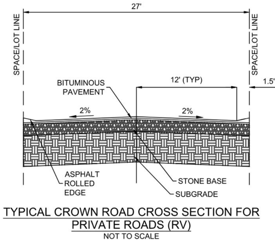
Figure 5 - Typical Crown Cross Section RV Private Roads
