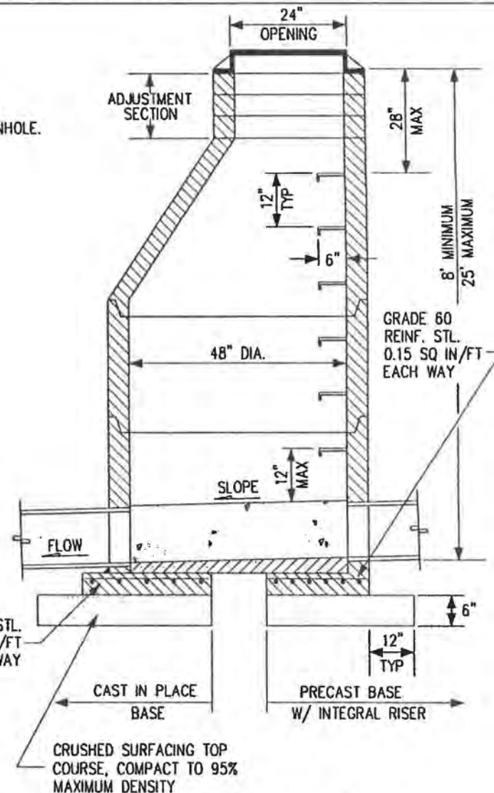
SECTION B-B
