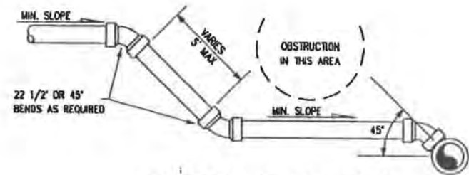
CONNECTION AT OBSTRUCTION
